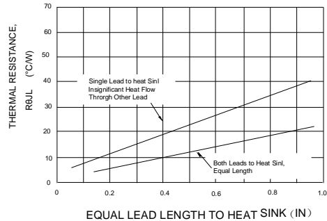
FIG.6-TYPICAL THERMAL RESISTANCE VS LEAD LENGTH
